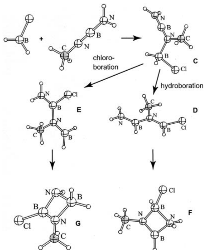
Figure 1. Optimised structures in the \text{BH}_2\text{Cl}/\text{H}_2\text{N}-\text{B}=\text{N}-\text{Me} system
