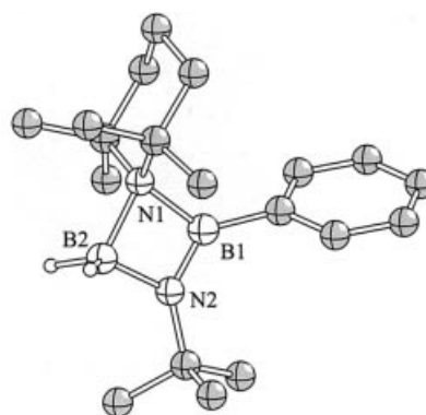
Figure 2. Optimised structure for \text{tmp}-\text{BPh}-\text{N}t\text{Bu}-\text{BH}_2 at the B3LYP/6-311G level of theory
